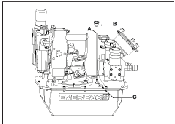
Figur 2, ZA4T-ventilatormontering
